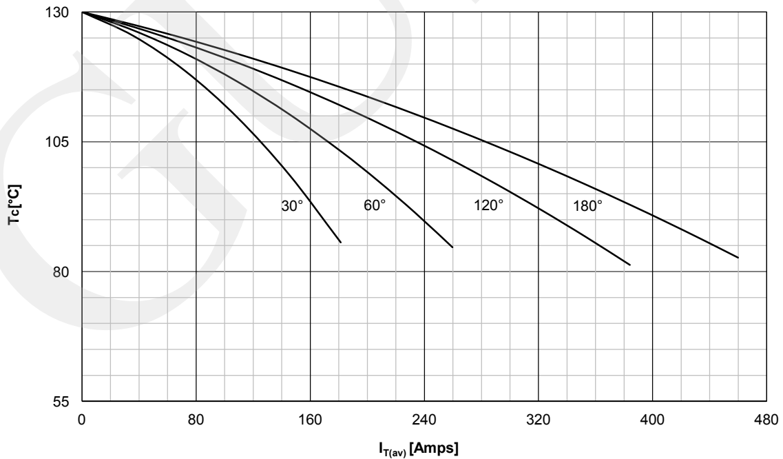
ON STATE CURRENT DERATING CURVE PER ARM SINE WAVE
